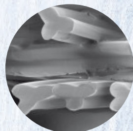
Cross section of trilobal filament
